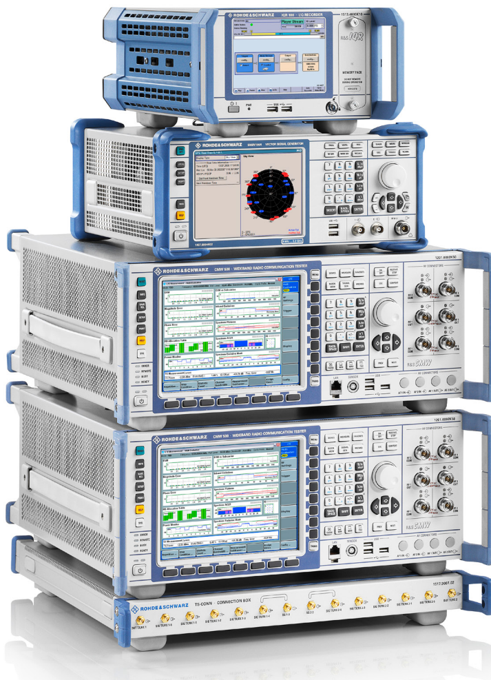
The R&S®TS-LBS advanced test system including carrier acceptance testing
